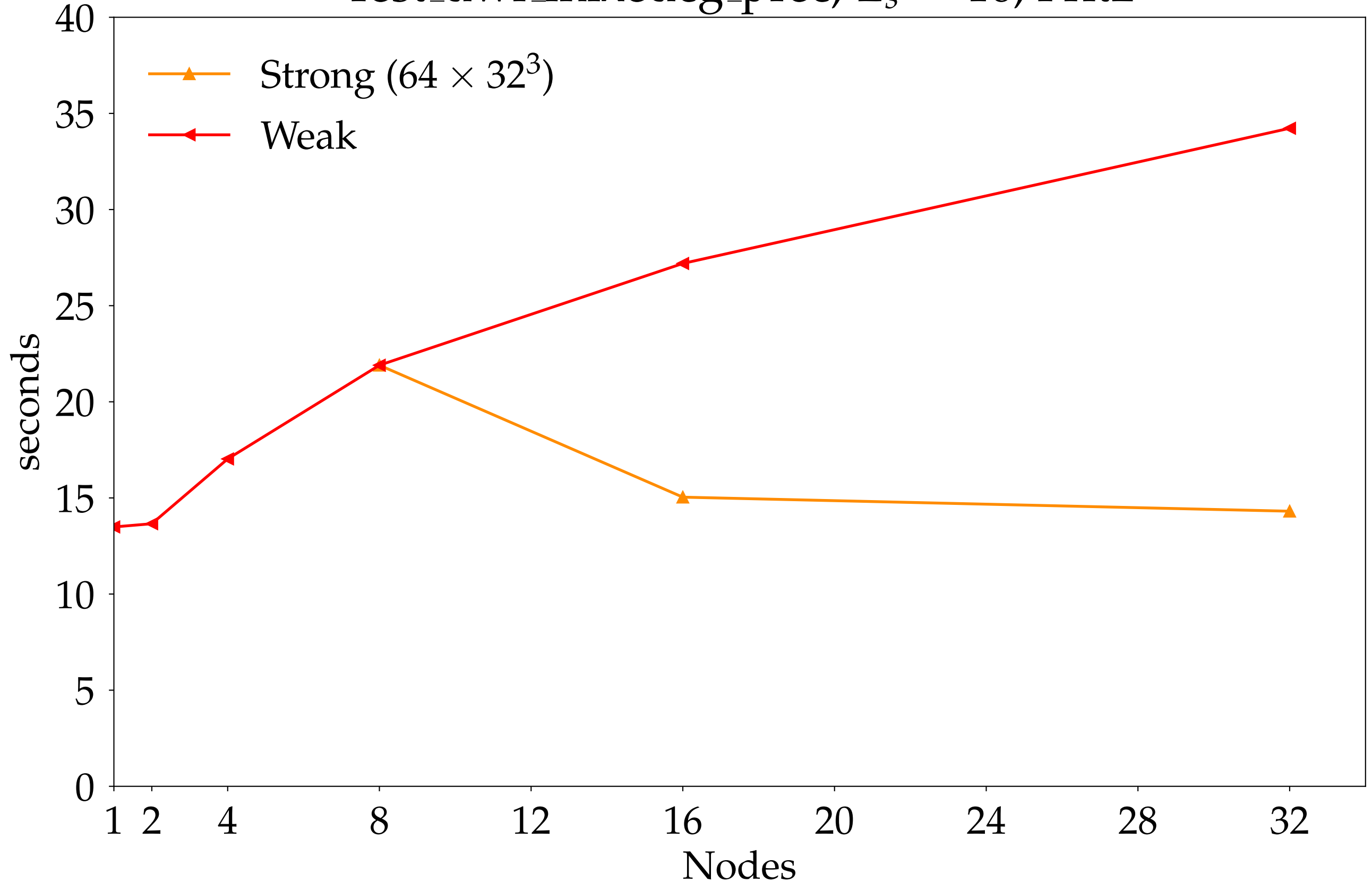
Test_dwf_mixedcg_prec, L_s = 16 , Fritz
