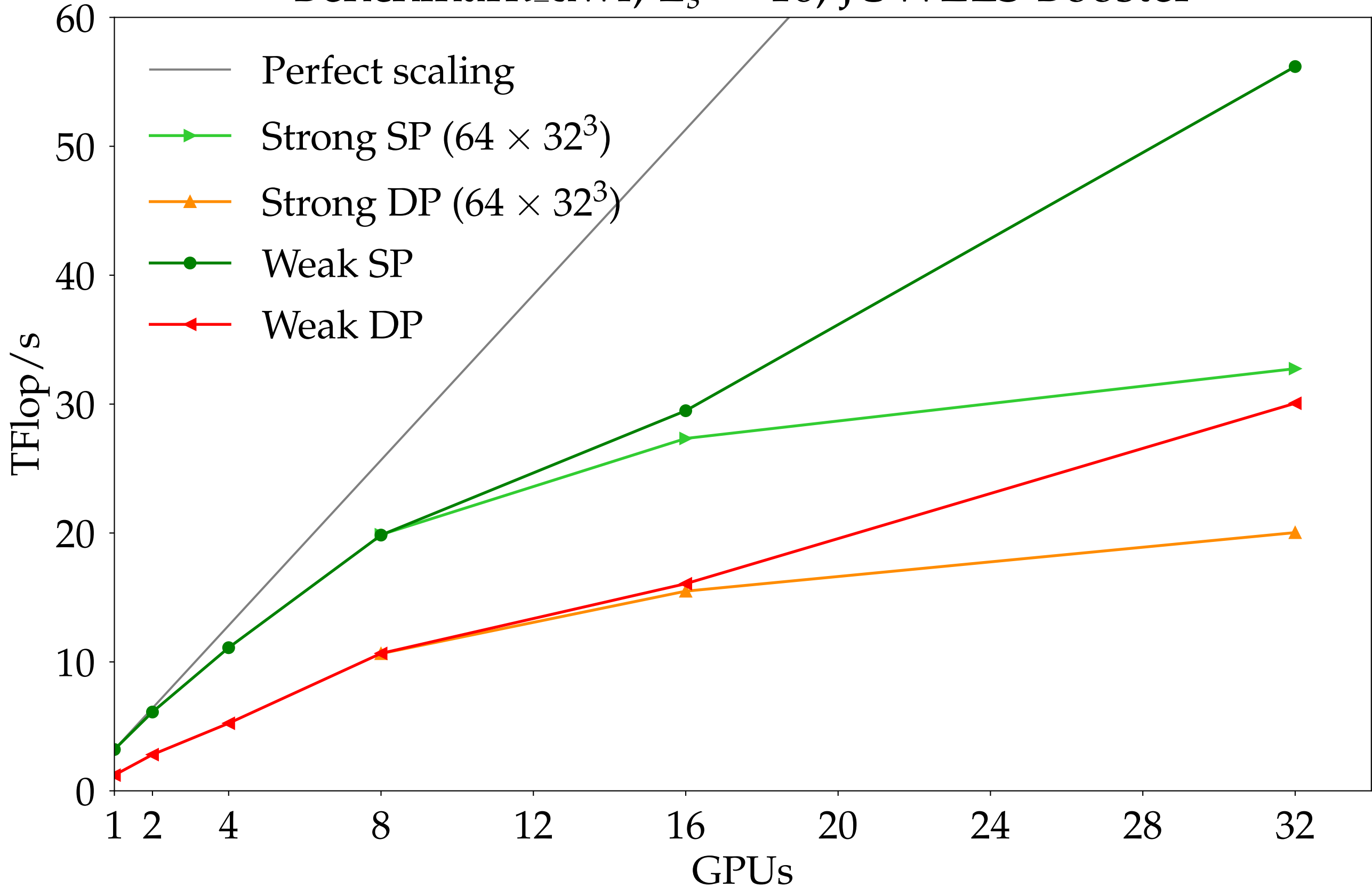
Benchmark_dwf, L_s = 16 , JUWELS Booster
