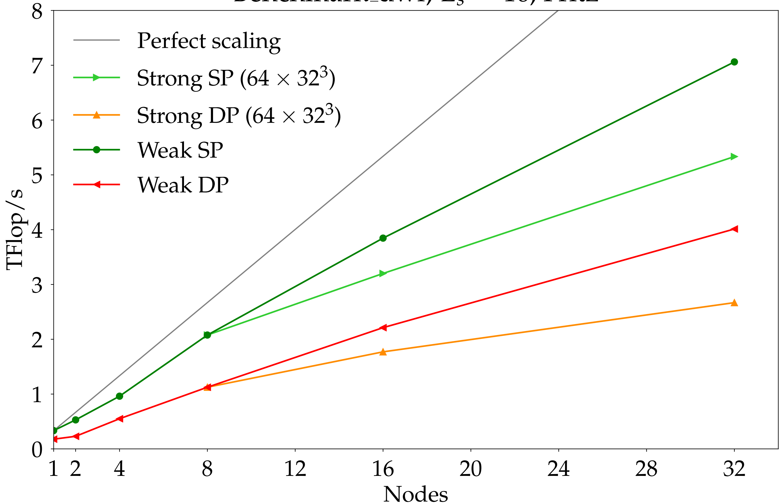
Benchmark_dwf, L_s = 16 , Fritz
