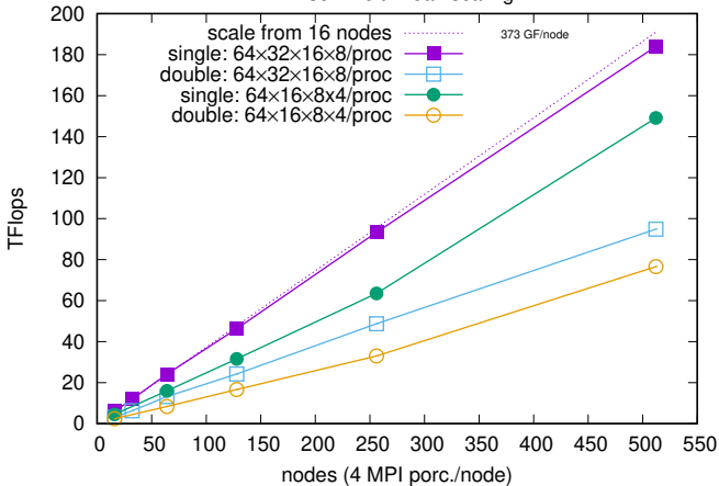
Wilson mult: weak scaling
