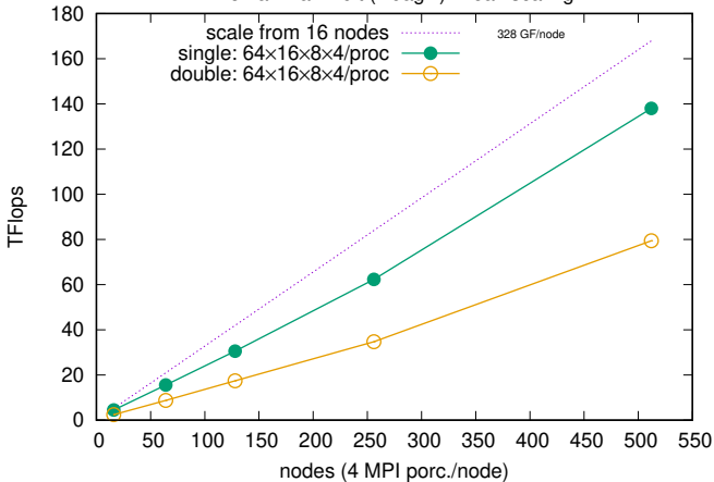
Domainwall mult (DdagD): weak scaling
